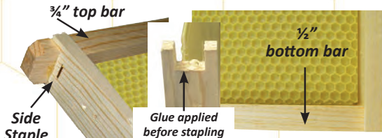
Close-up of assembled frame construction top bar and bottom bar.
